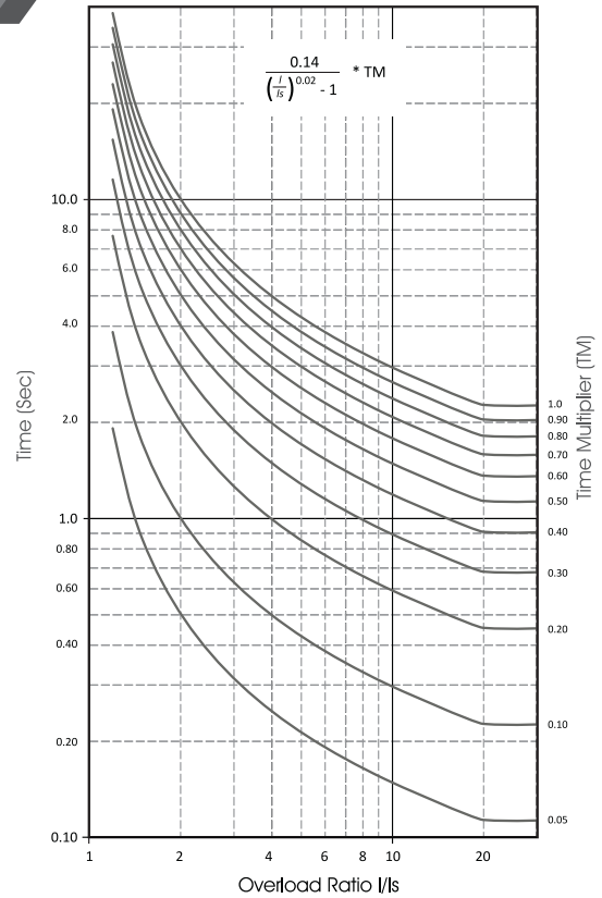
normal inverse 1.3
