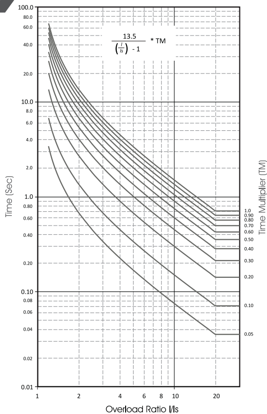
very inverse
