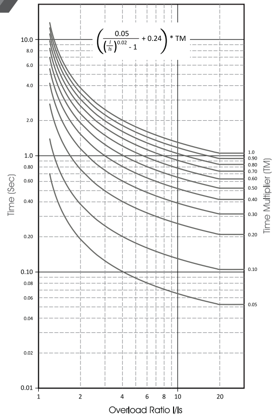
normal inverse 1.3
